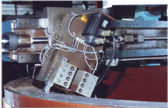
Insitu Flange Facer - for Shell Machining
