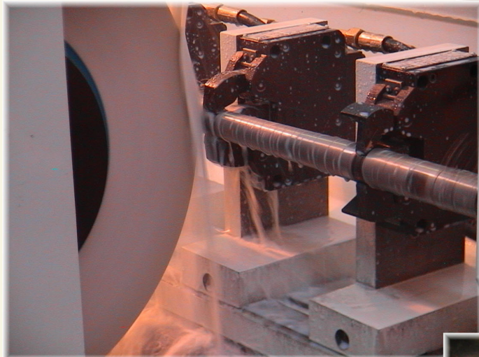
Pilger Mandrel Grinding Machine
