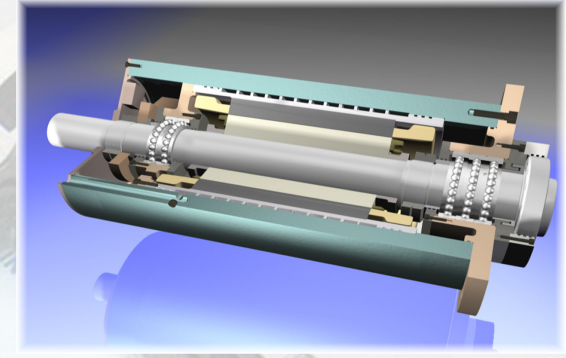
Motorized Spindle - for Machining Centres
